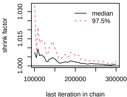
d.chemo.Gefitinib
