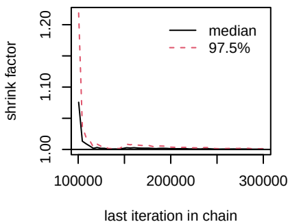
d.chemo.Afatinib
